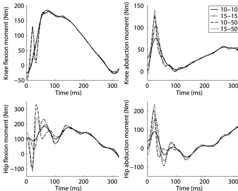
Fig. 3. External joint moments (Nm) for a typical player with different combinations of cut-off frequencies for the filtering of force and movement data. A-B: A and B refer to cut-off frequency for marker and force data respectively.
